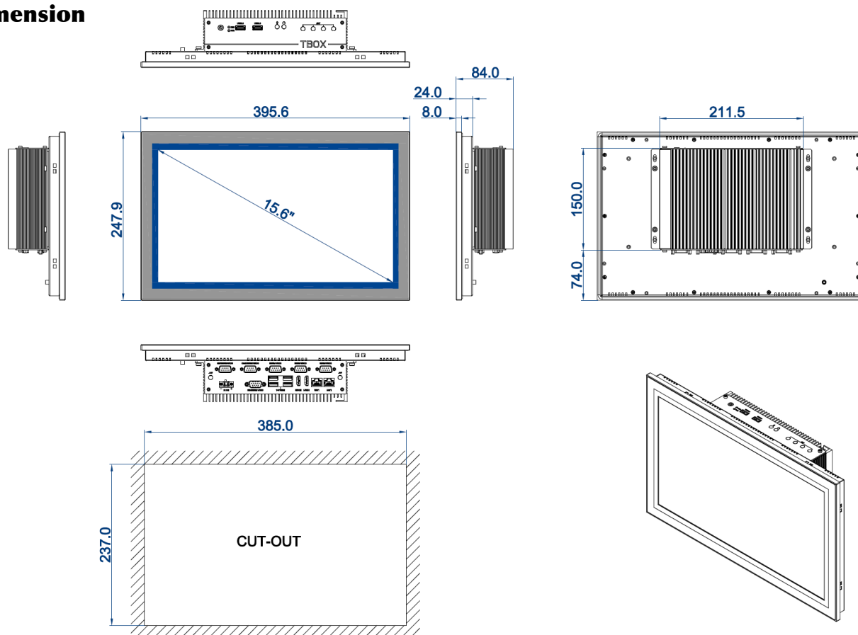
DIMENSIONAL DRAWING:TPC-PRS156A/W
