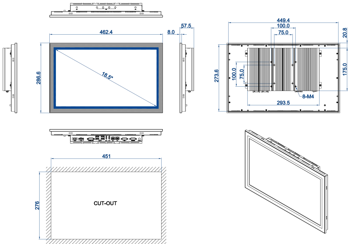
DIMENSIONAL DRAWING:TPC-DRS185
