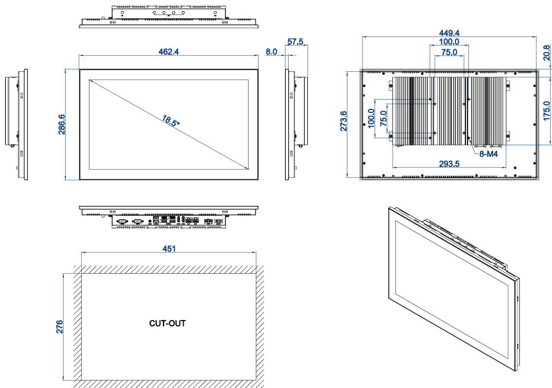
DIMENSIONAL DRAWING:TPC-DCS185E1
